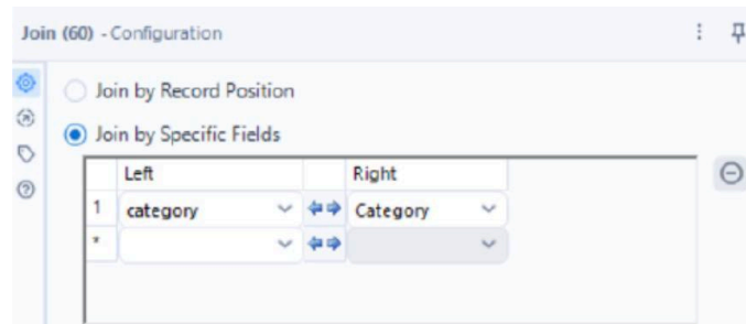
Figure 2.3 Join 2 configuration panel, join condition: merged.category=DS3_agg.Category
